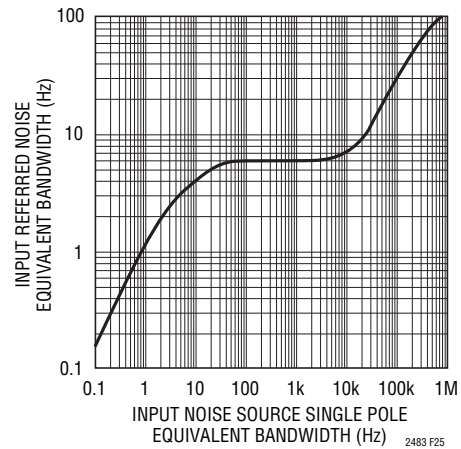
Figure 25. Input Referred Noise Equivalent Bandwidth of an Input Connected White Noise Source
